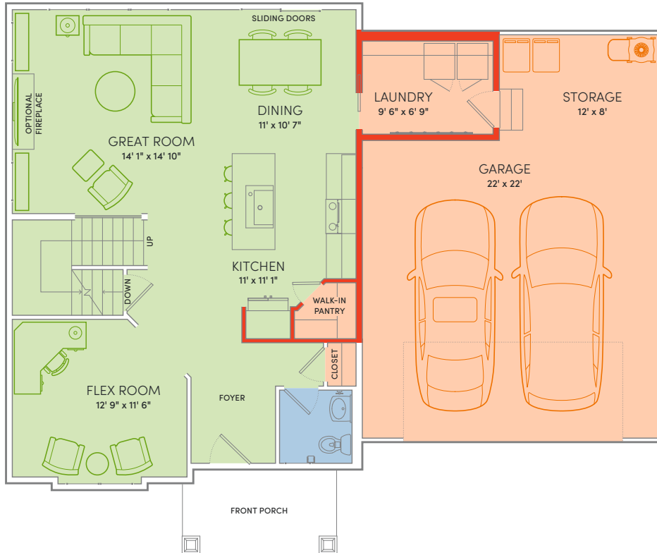
STANDARD PLAN: WALK-IN KITCHEN PANTRY & LAUNDRY ROOM OFF GARAGE
