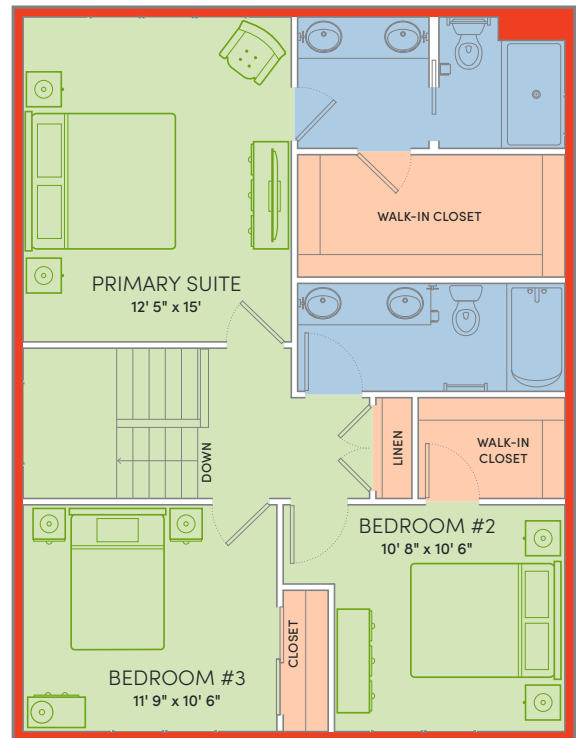
REVISED 3-BEDROOM OPTION
