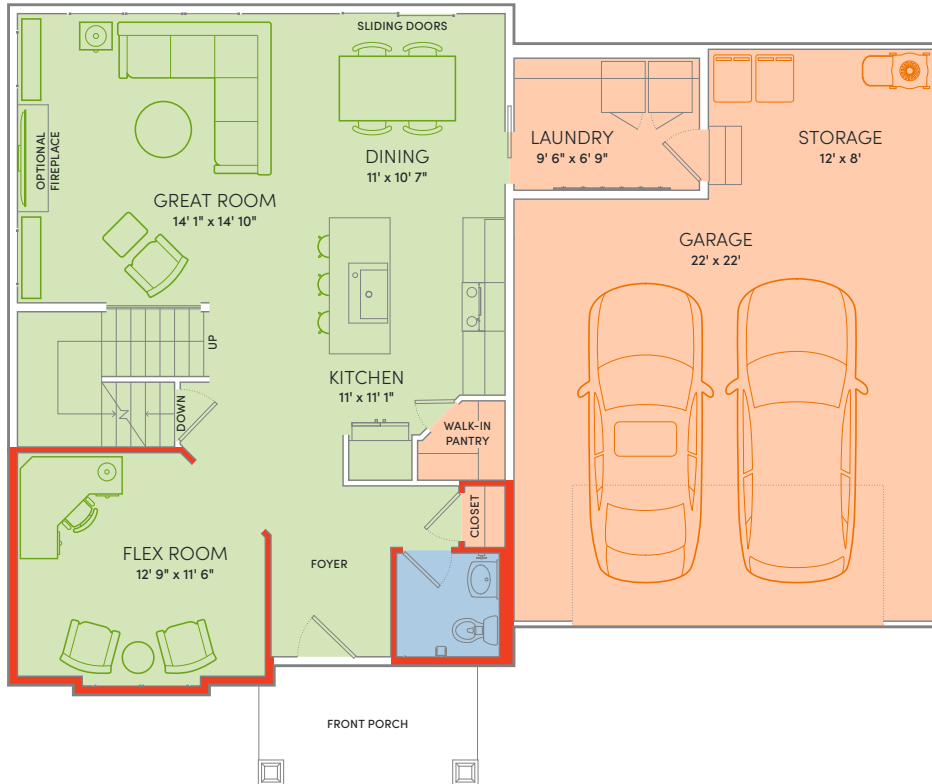
STANDARD PLAN: POWDER ROOM, FOYER CLOSET & FLEX ROOM
